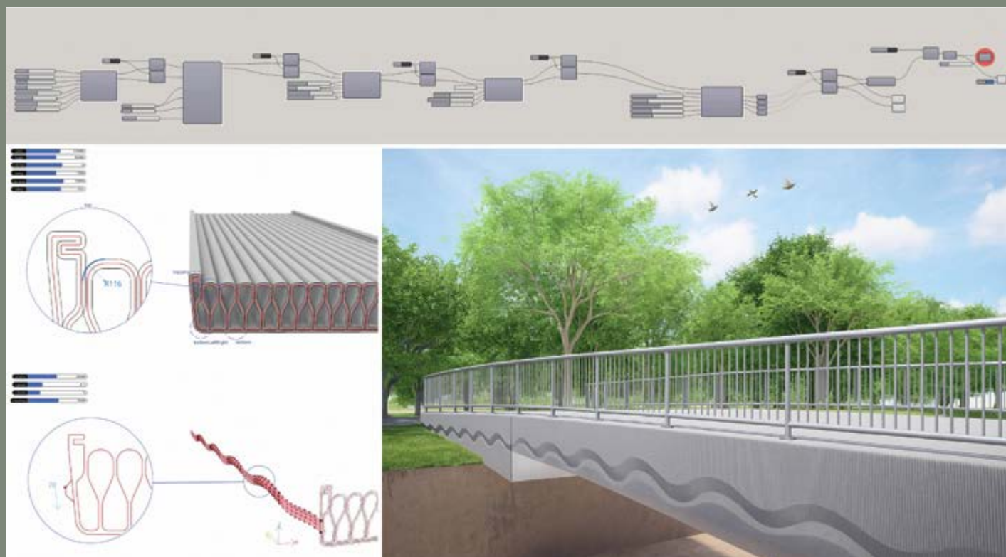
Singapore 3DCP load bearing bridge. Bron: Witteveen+Bos
